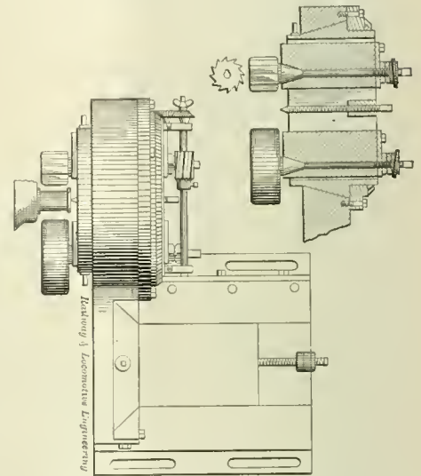
CRANK PIN TURNING MACHINE.
